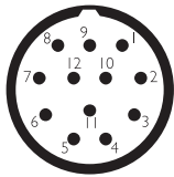
M23-Steckverbinder, 12-polig
