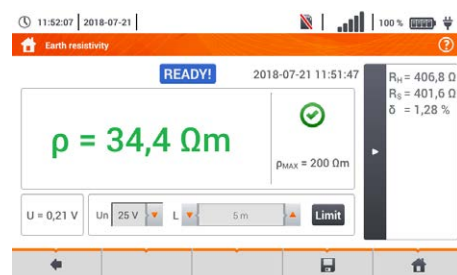
Ground resistivity measurement
